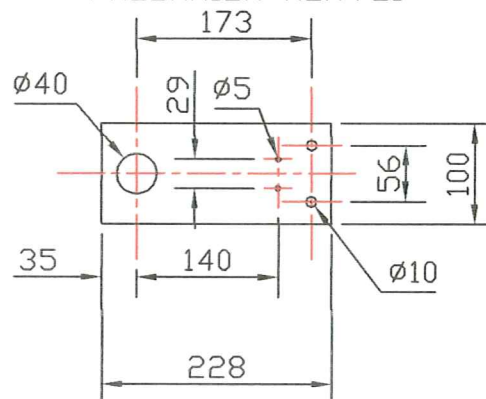
DETAIL PALONNIER RENVOI
