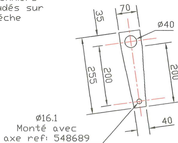
DETAIL PALONNIER B.A.R.
